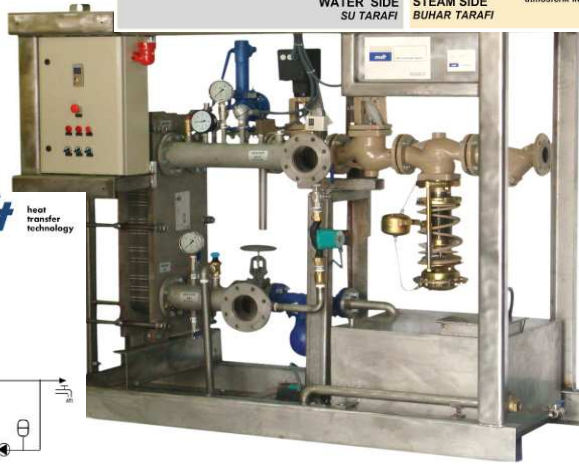
STATION-FLUID HEATING BY HOT WATER-4
