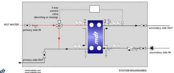
STATION-FLUID HEATING BY HOT WATER-4
