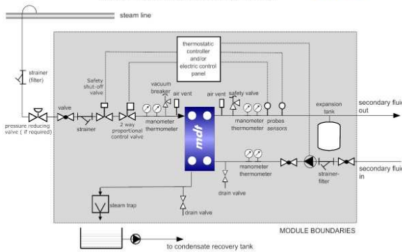
COMPACT MODULE-WATER / LIQUID heating BY STEAM
